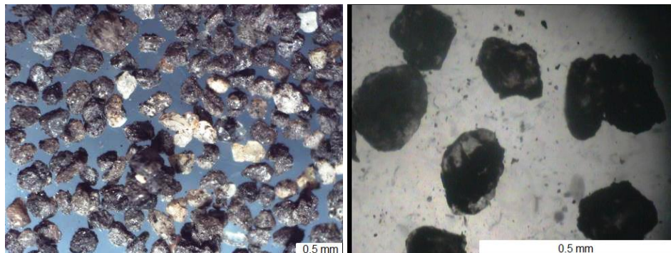
Fig. 1. Optical microscope photographs of waste foundry sand.
