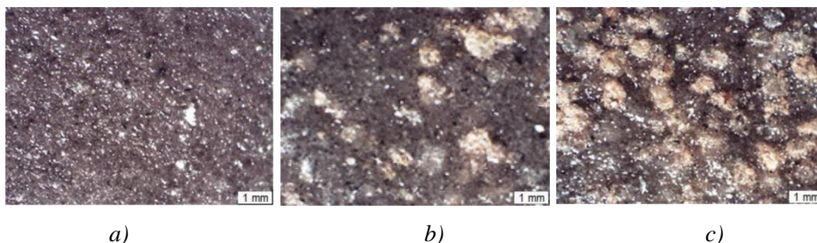
a) b) c) Fig. 4. Surface textures of samples sintered at T = 750\text{ }^{\circ}\text{C} for t = 1\text{h} : a) WGS; b) WGS 30 c) WGS 50.
