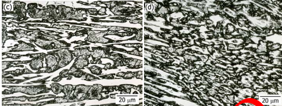
Fig. 4. Optical micrographs of Fe-Cr-C alloy (a) and Fe-Cr-C-V alloy containing 2.02% V (b), 3.28% V(c), 4.73% V (d) in the heat treated state (500°C/4h).
